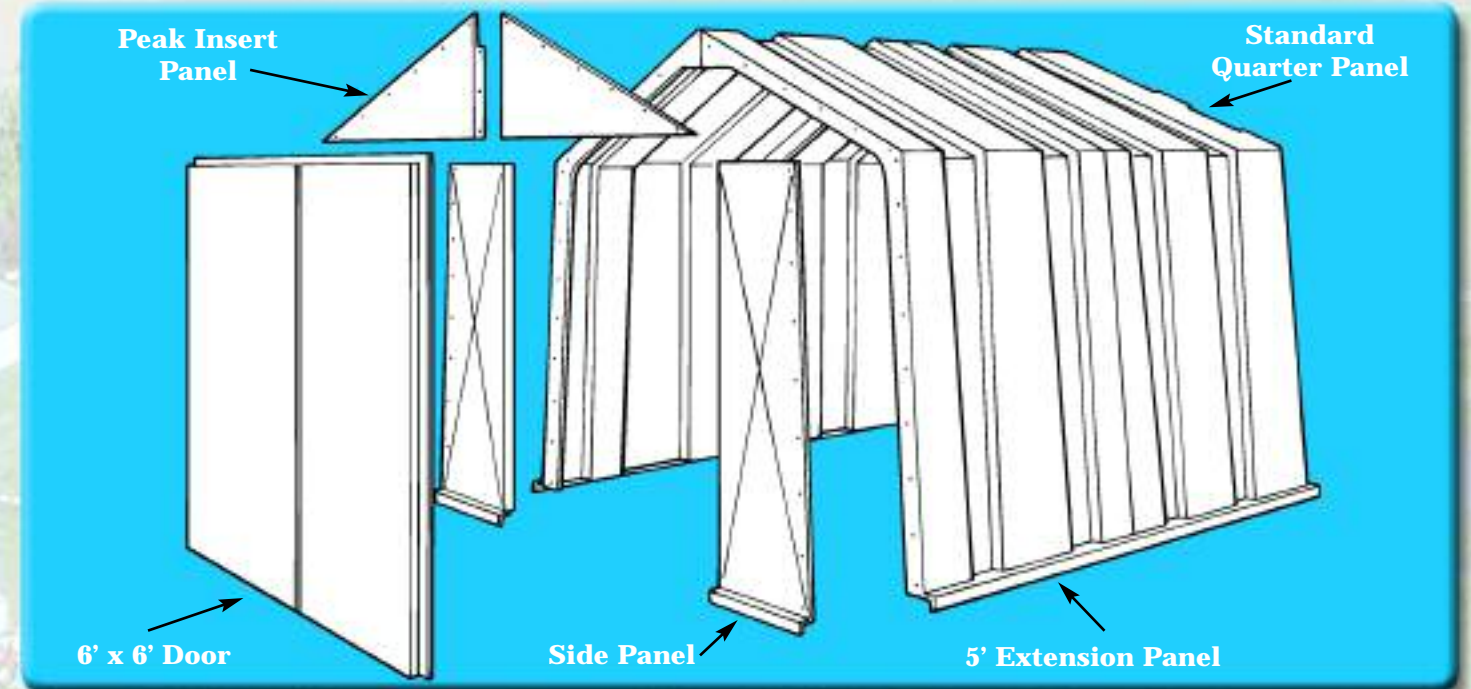
Assembly view of Mega Hut with optional 6' x 6' door kit
