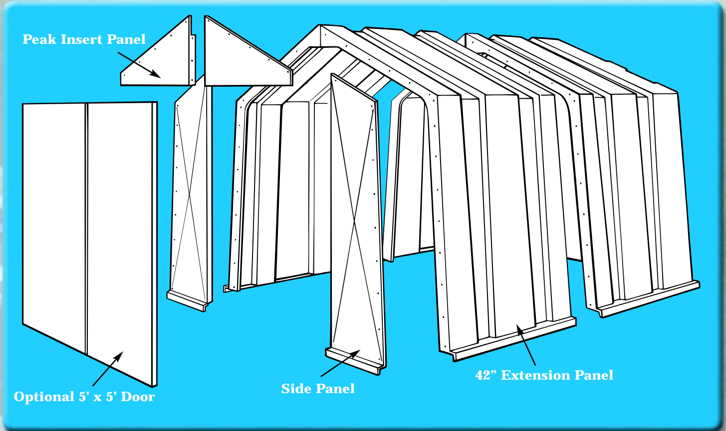
Assembly view of Super Hut with optional 5' x 5' door kit
